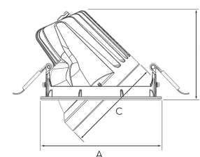
A= 158mm B= 122mm C= 121.5mm
